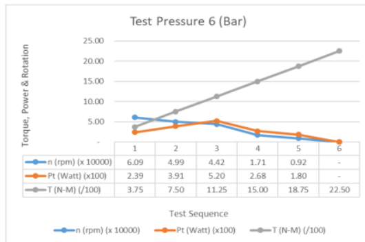
Figure-4. Graph between Torque, Power, Rotation with interval of data collection at pressure 6 (bar).
