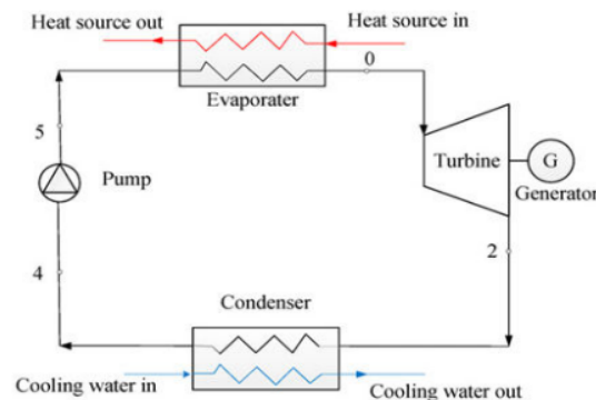
Figure-1. Organic rankine cycle system.
