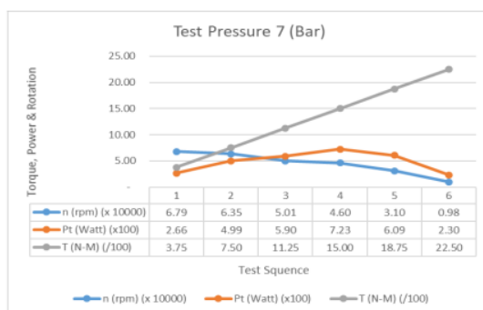
Figure-5. Graph between Torque, Power, Rotation with time interval for taking data at pressure 7 (bar).
