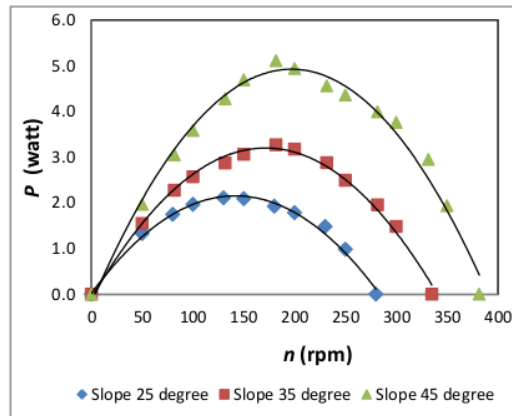
Figure-5. Rotation vs. output power of screw turbine at y = 1R_o and c_o = 0,5 m/s.
