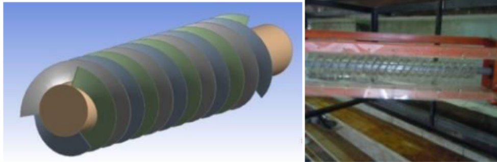
Figure-1. Model of three-bladed Archimedes Screw turbine[15].
