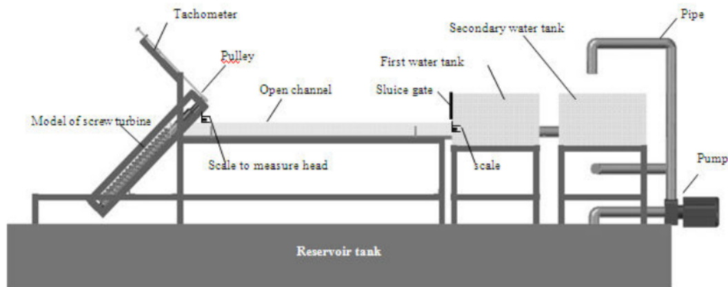
Figure-2. Archimedes screw turbine installation[15].
