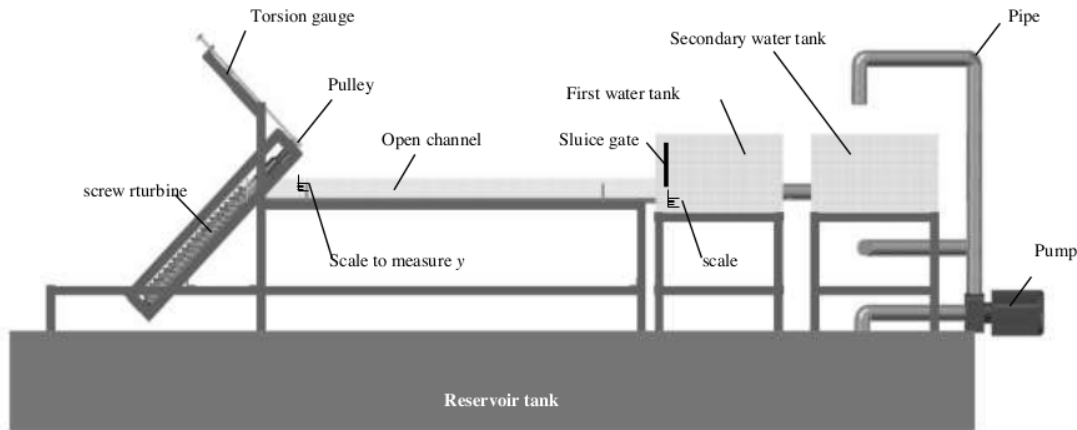
Figure 2. The screw turbine Installation [12], [13]
