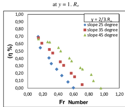
Figure 7. Shaft declivity effect toward Fr and efficiency at y = 2/3.R_o
