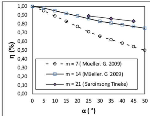
Figure 9. The experimental results and the results of [4]
