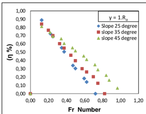
Figure 6. Shaft declivity effect toward Fr and efficiency
