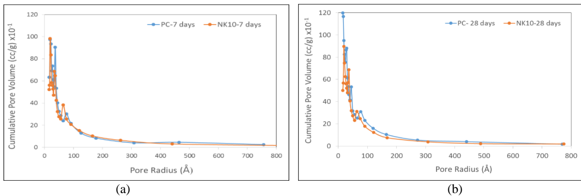
Figure 6. Cumulative pore volume vs pore radius of cement paste with and without nano-metakaolin at (a) 7 and (b) 28 days
