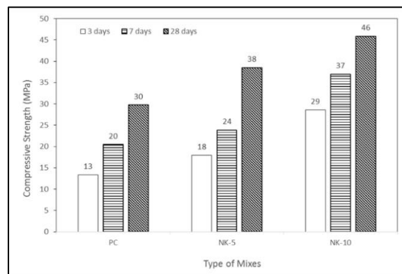
Figure 3. Compressive strength of cement concretes with nano-metakaolin at 3, 7 and 28 days
