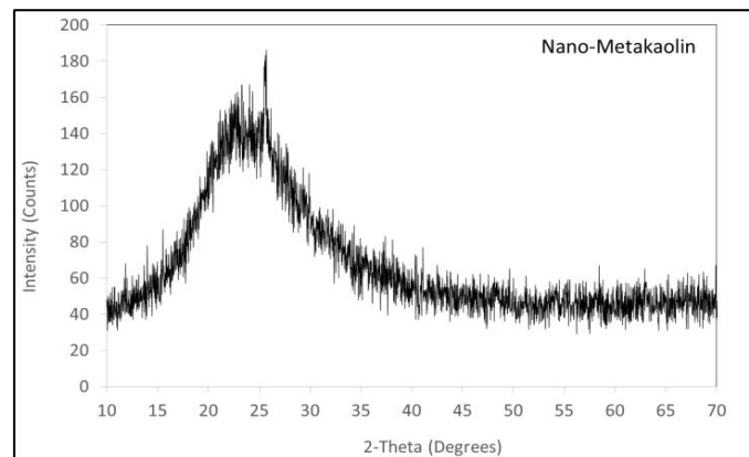
Figure 1. X-Ray Diffraction of nano-metakaolin
