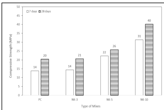
Figure 2. Compressive strength of cement mortars with nano-metakaolin at 7 and 28 days
