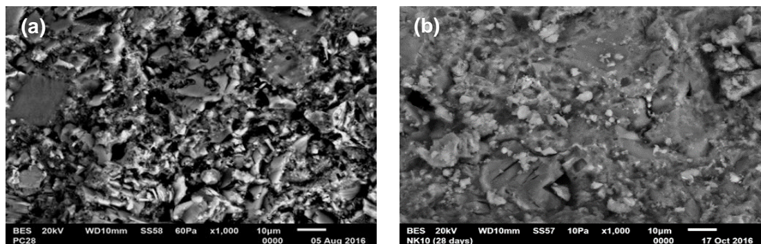
Figure 4. Backscattered Electron images of (a) cement paste and (b) cement paste with nano-metakaolin at 28 days
