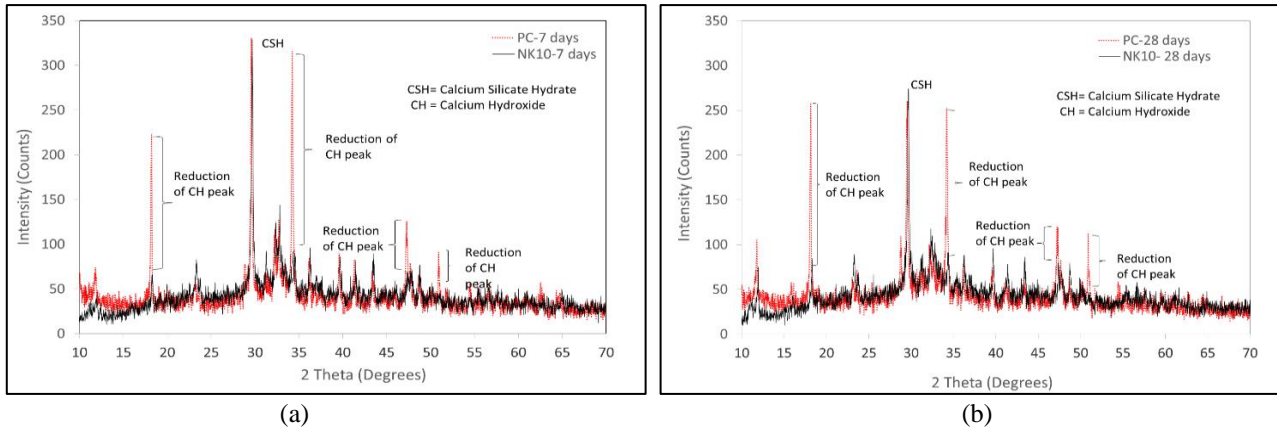
Figure 5. XRD analysis of cement paste with and without nano-metakaolin at (a) 7 days and (b) 28 days
